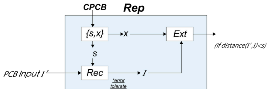
Figure: CPCB Matching Verification
