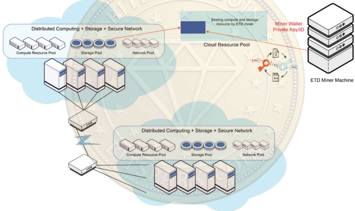
Figure: BTK Overall Technology Framework
