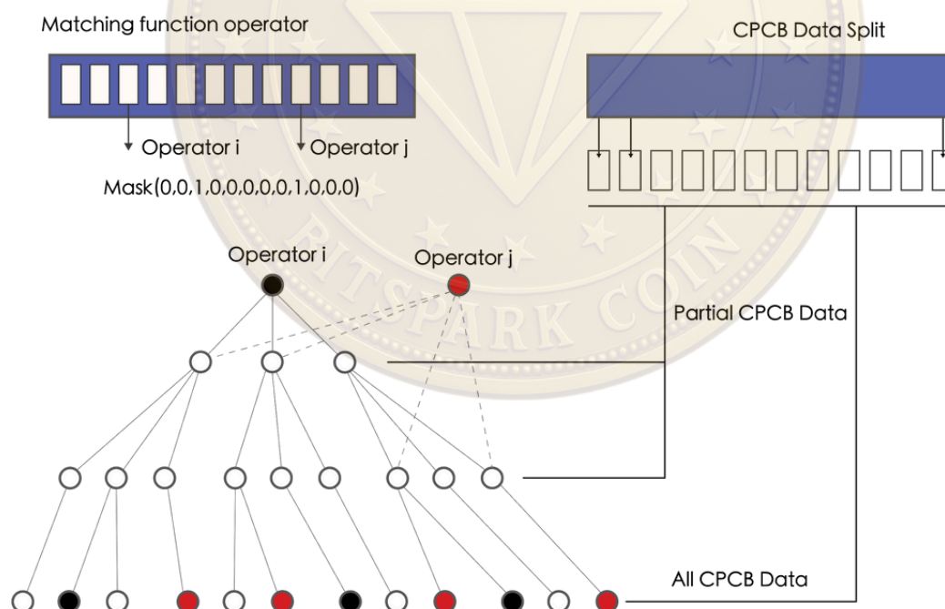
Figure: Double Blind Matching Operators
