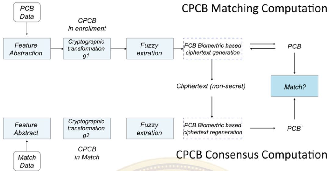
Figure: Double blind matching system framework
